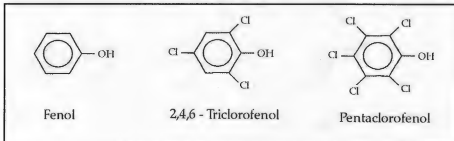
FIGURA 1. Fenoles
