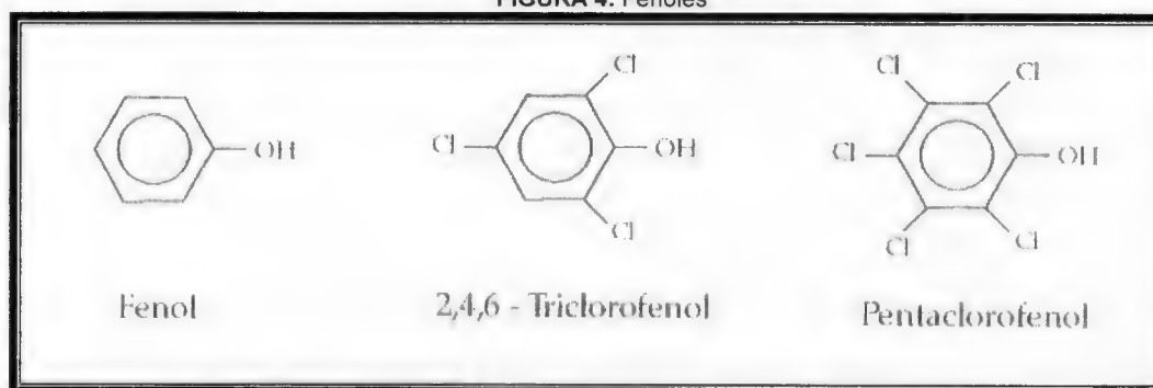
FIGURA 4. Fenoles
